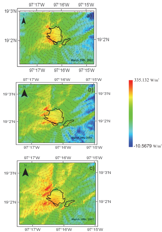
Fig. 5. Net radiation distribution over Glaciar Norte's surface derived from ASTER imagery. The highest values are observed in March 2007 (c). Observe the strongest values of net radiation on the western part of the glacier. (a, c).
