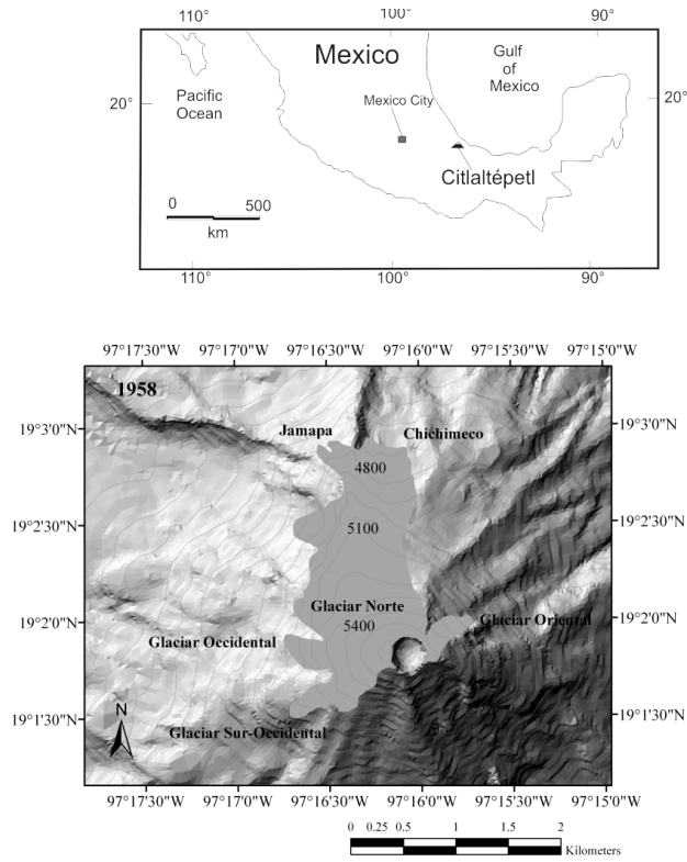
Fig. 1. Location of Citlaltépetl Volcano and extent of the glaciers documented in 1958 by Lorenzo (1964).
