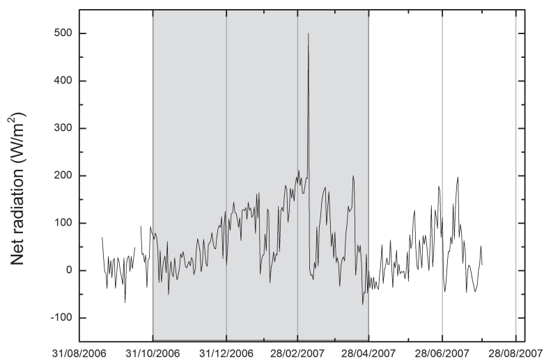
Fig. 4. Net radiation variability of the Glaciar AWS data from September 2006 to July 2007 (after Ontiveros-González, 2007).
