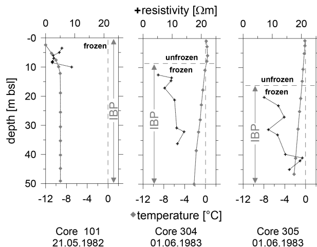
Figure 4. Water electrical resistivity and temperature are shown for: (a) bottom water measured for the period 1 September 2008 – 31 August 2009 in 7.2 m water depth and (b) for sediment pore water from cores recovered from boreholes 101, 304 and 305 on the dates indicated (Figs. 1 and 3; Table 1).
