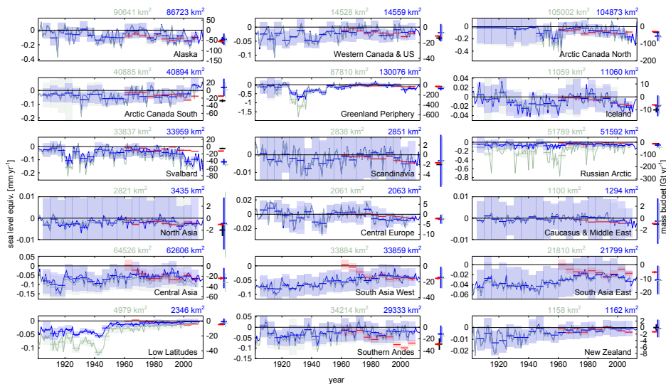
Figure 2. Regional glacier mass change rates, colors as in Fig. 1. Shading indicates the 90 % confidence interval of the pentadal means. Numbers given on top of each panel indicate glacier area in RGIv1.0 (green) and RGIv4.0 (blue). Crosses on the right of each panel give mass change rate and 90 % confidence interval during 2003–2009.
