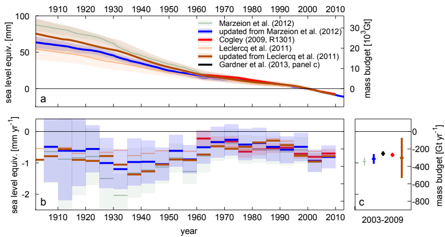
Figure 1. Globally integrated glacier mass change; (a) accumulated in time, relative to the year 2000; (b) pentadal mean values of mass loss rates; (c) mean mass loss rates during 2003 to 2009. Shading/error bars indicate 90 % confidence interval. Note that all reconstructions exclude glaciers in the Antarctic periphery.
