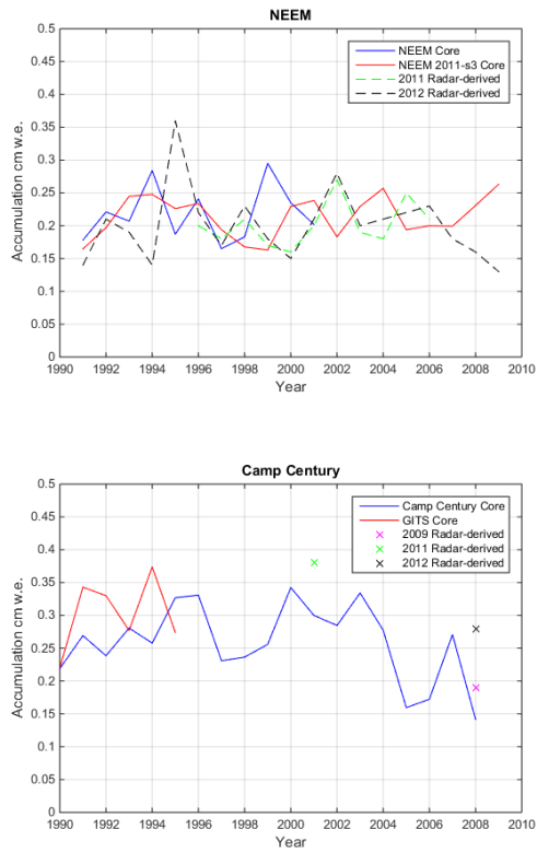
Figure 11. Annual accumulation rate measured from the two cores at both the NEEM and Camp Century locations compared to temporally overlapping radar-derived values.
