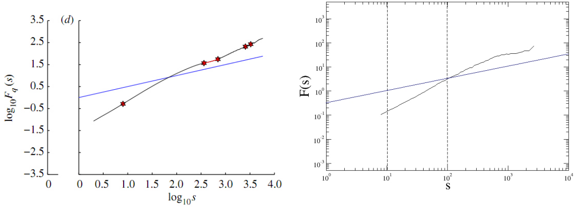
Figure 1: Left panel. TW-DFA curve ( q = 2 ) from the paper by Agarwal et al, deseasonalised equivalent ice extent. Right panel. DFA curve calculated using conventional DFA3. Dashed lines denote the time scale 10-100 where DFA-indicator is calculated as the slope of the DFA curve; in this time scale DFA and TW-DFA curves have the same \alpha .
